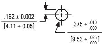
Mounting Detail (Single Pole and Two Pole)
