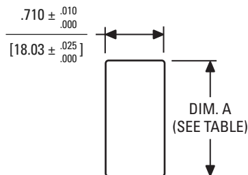
Mounting Detail
