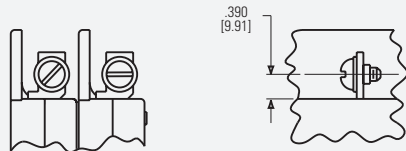
10 - 32 or 1/4 - 20 Screw Terminals
